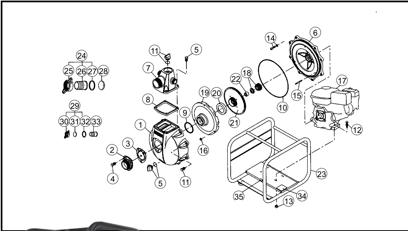
2" HIGH PRESSURE MITSUBISHI GM182 6.0 HP
