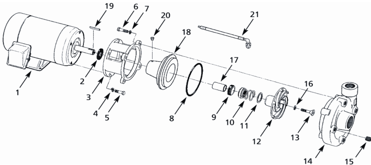
Figure 1 - Repair Parts Illustration Repair Parts List
