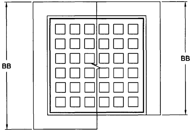
4 - SIDED FRAME 3 - SIDED FRAME
