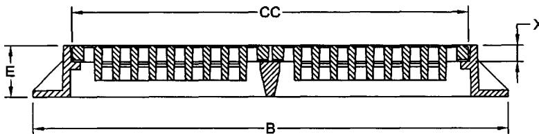
4 - SIDED FRAME
