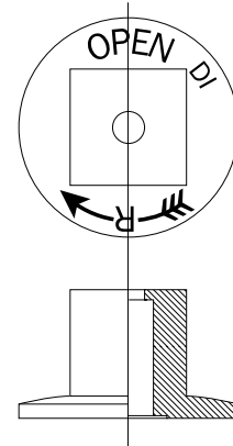
Fig. No. HON-01 Hydrant Operating Nut Weight - 2 lbs.
