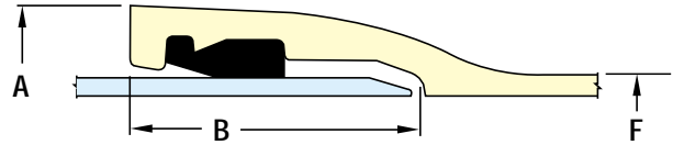
FASTITE JOINT® Pipe 30" — 48"
