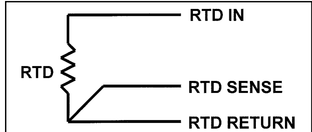
FIGURE 10-3. Three-Wire RTD Configuration.
