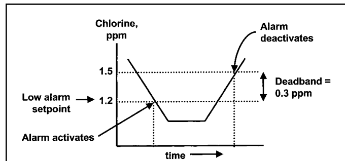
FIGURE 7-2. Low Alarm Logic
