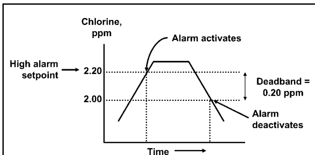
FIGURE 7-1. High Alarm Logic
