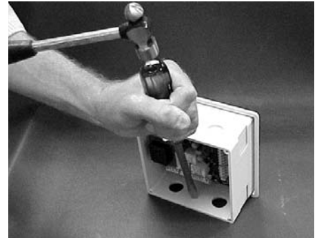
FIGURE 4-1. Removing the Knockouts
